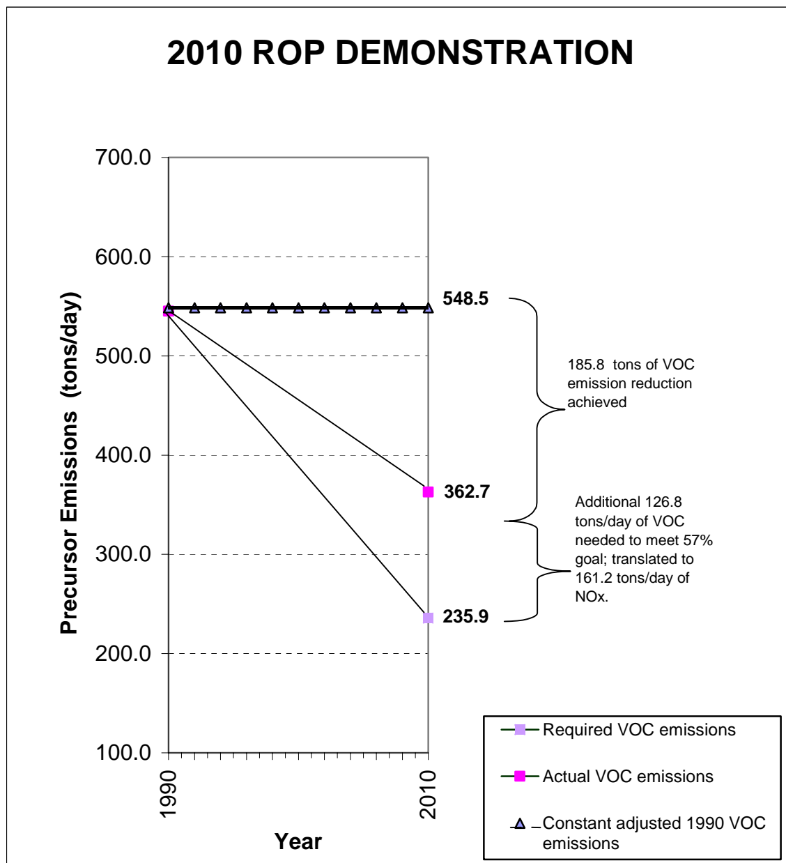
Figure 7-2 Graphical Summary of 2010 ROP Demonstration for San Joaquin Valley Ozone
